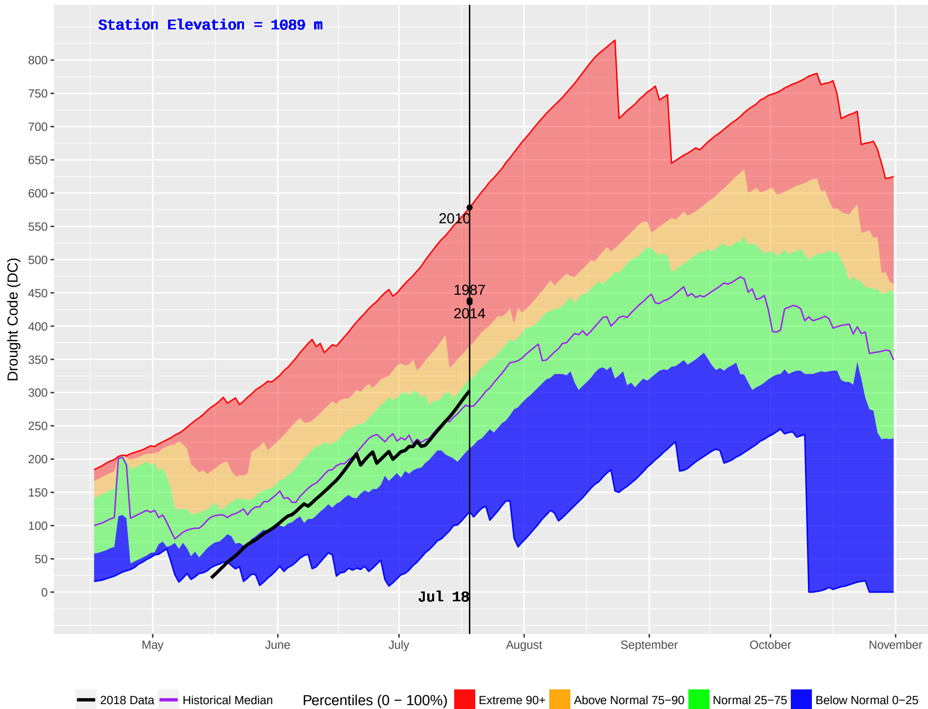
EAST OOTSA (170) : Historical (1986–2016) and Current (2018) Daily Drought Code (DC)
